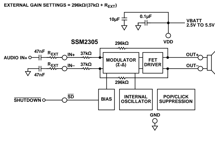
Figure 33. Single-Ended Input Configuration, User-Adjustable Gain
