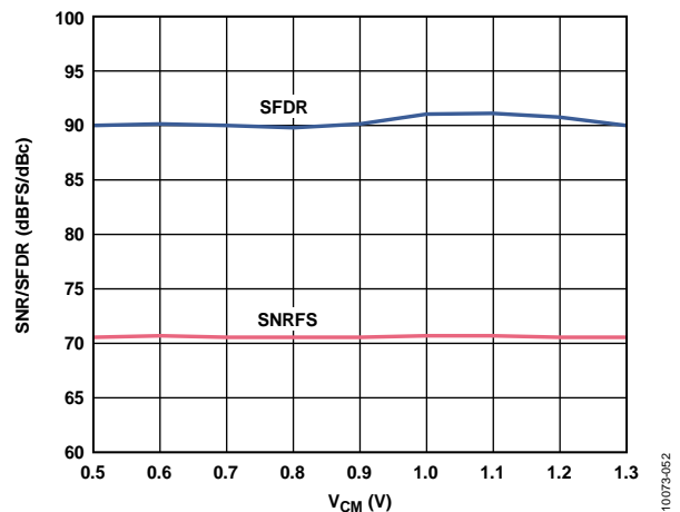
Figure 55. SNR/SFDR vs. Common-Mode Voltage, f_{IN} = 9.7 \text{ MHz} , f_{SAMPLE} = 125 \text{ MSPS}
