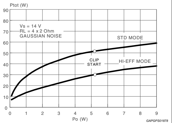
Figure 18. Power dissipation vs. average output power (audio program simulation, 2 Ω)
