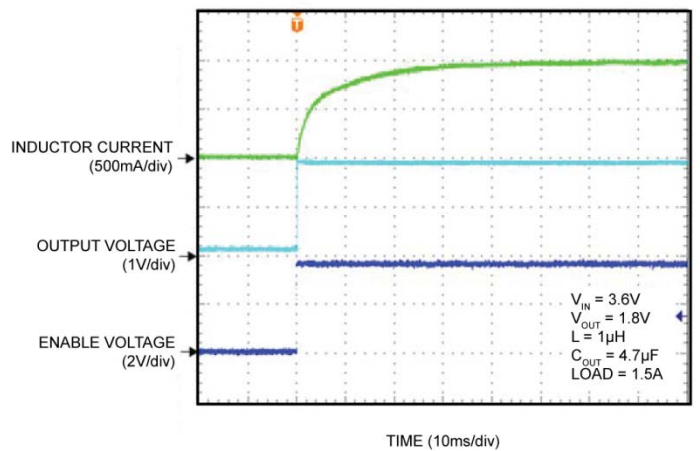
Start-Up Waveform
