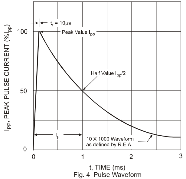
Fig. 4 Pulse Waveform
