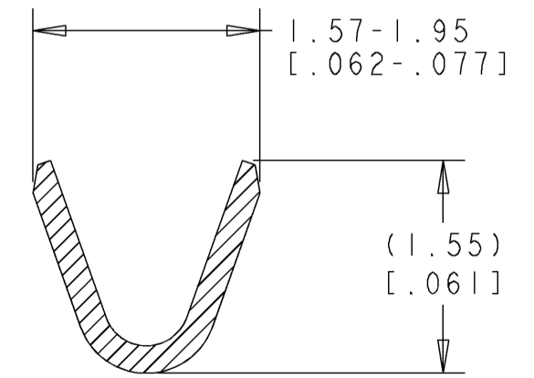
SECTION B-B SCALE 20:1
