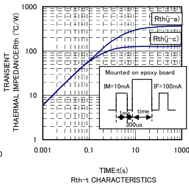
Rth-t CHARACTERISTICS
