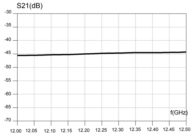
Figure 8. Attenuation 5f0 (dB)
