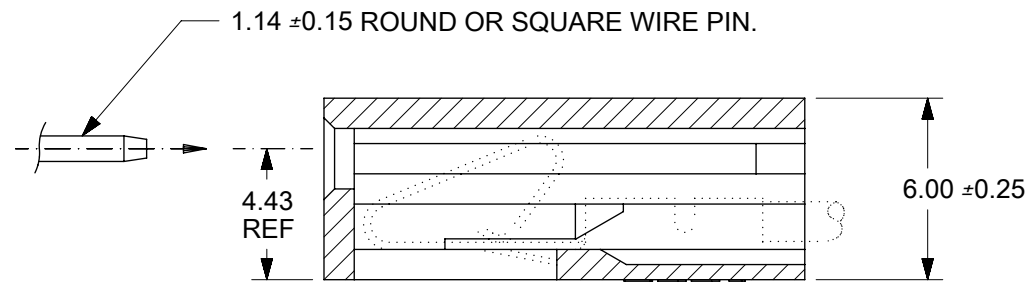
SECTION Z-Z
