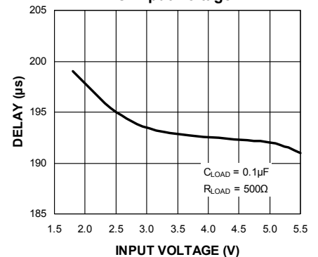
Output Turn-On Delay vs. Input Voltage
