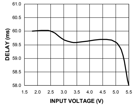
Output Turn-On Delay vs. Input Voltage
