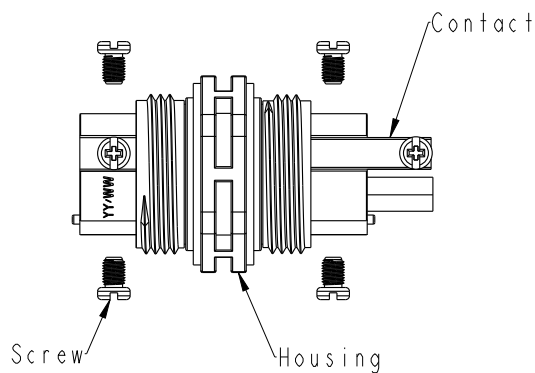
6 Connector
