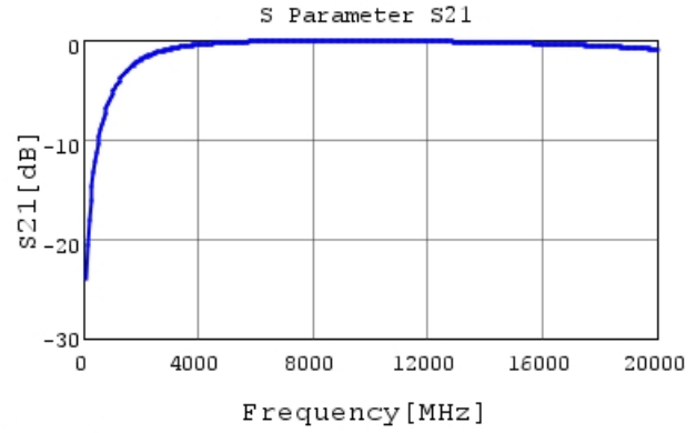
GRM0335C1H1R0CA01 S21 DCOV, 25degC
