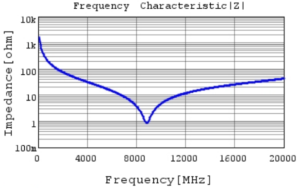
GRM0335C1H1R0CA01 |Z| DCOV, 25degC
