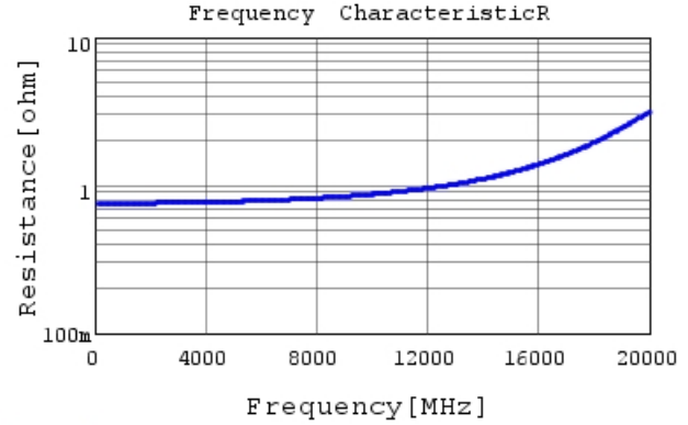
GRM0335C1H1R0CA01 R DCOV, 25degC
