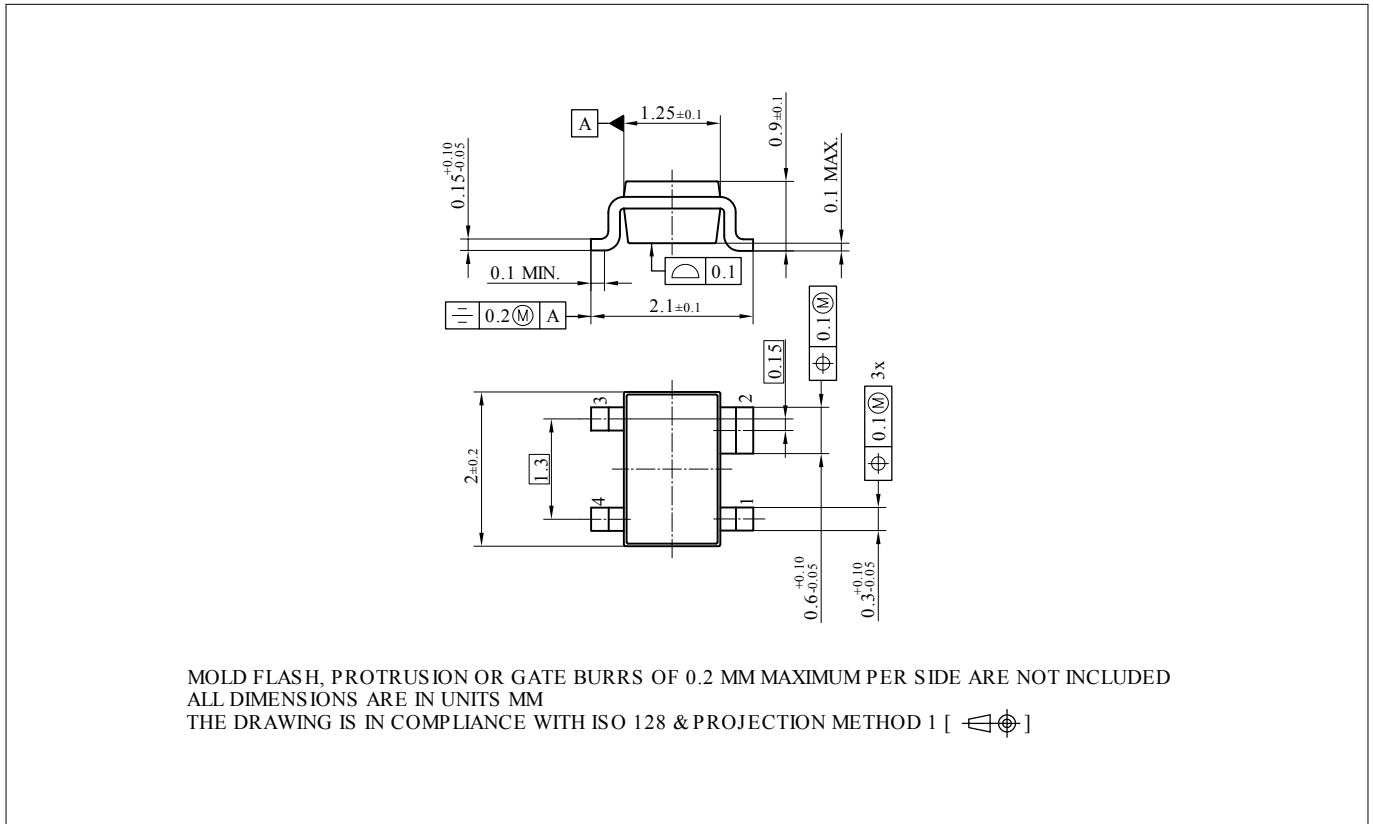
Figure 20 SOT343 package
