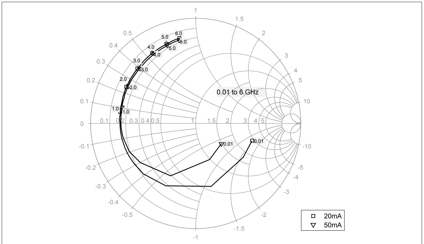
Figure 14 Input reflection coefficient S_{11} = f(f) at V_{CE} = 8 V, I_C = 20, 50 \text{ mA}
