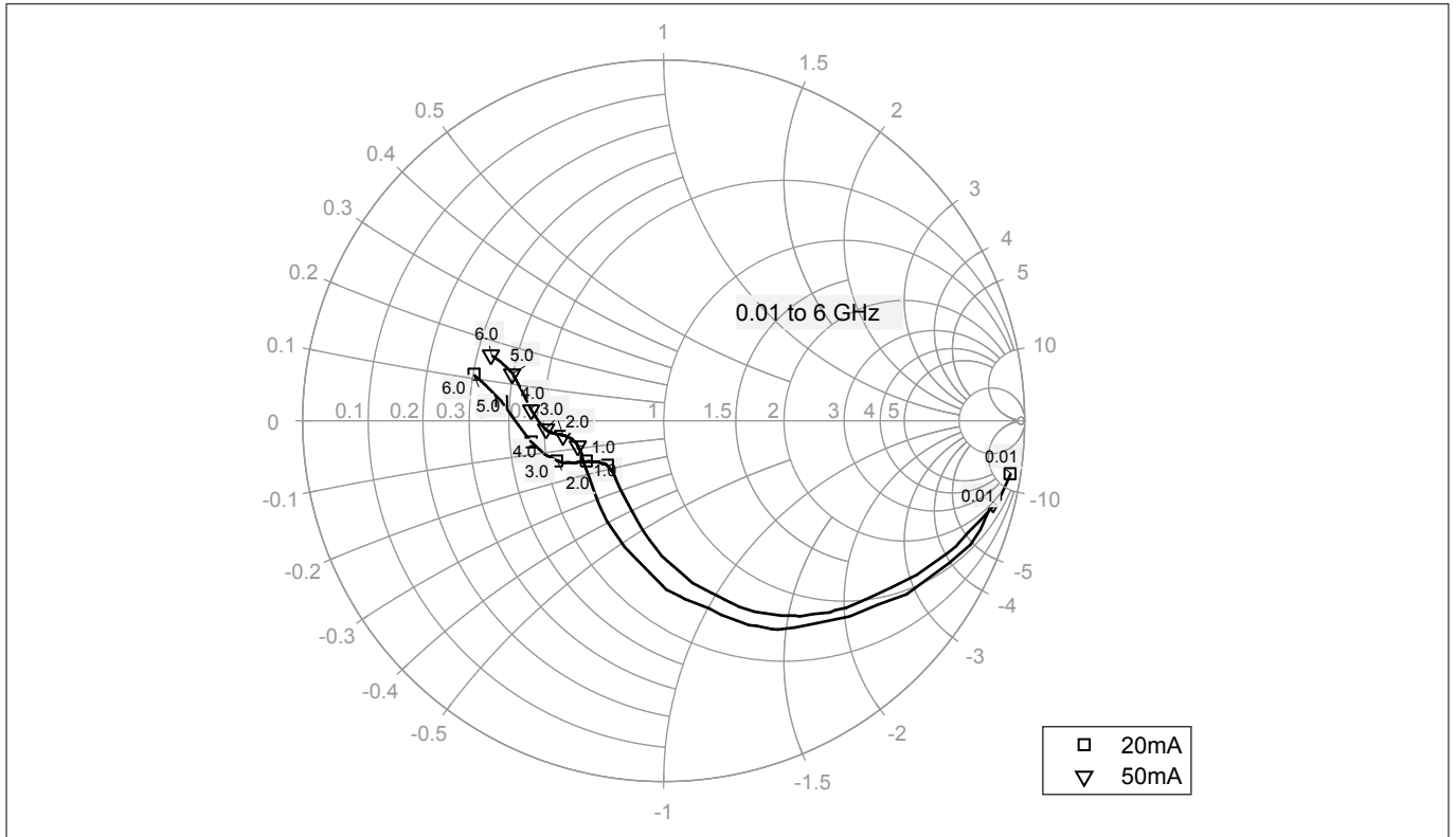
Figure 13 Output reflection coefficient S_{22} = f(f) at V_{CE} = 8 V, I_C = 20, 50 \text{ mA}
