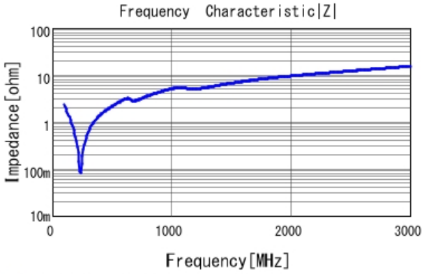
■ GRM31A5C2J561JW01 |Z| DCOV, 25degC
