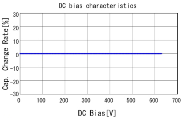
■ GRM31A5C2J561JW01 C-DC bias capchange, 25.0degC, AC1V
