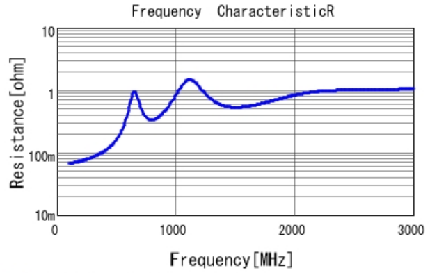
■ GRM31A5C2J561JW01 R DCOV, 25degC
