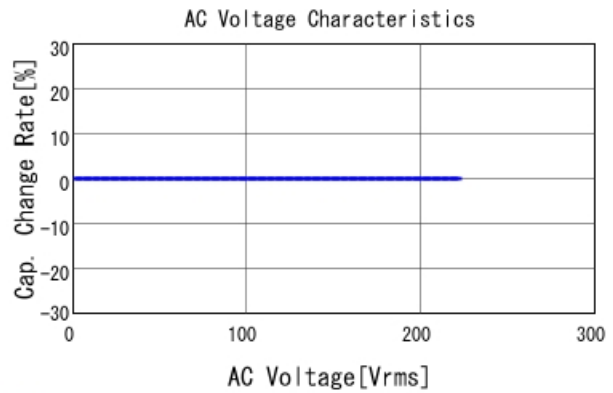
■ GRM31A5C2J561JW01 C-AC Voltage capchange, DCOV, 25.0d
