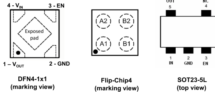
Figure 2. Pin configuration
