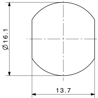
Mounting hole ML 12
