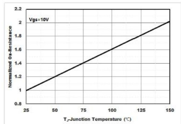
Figure6. Normalized On-Resistance
