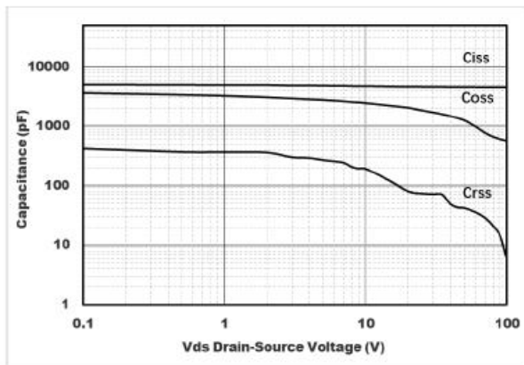
Figure3. Capacitance Characteristics
