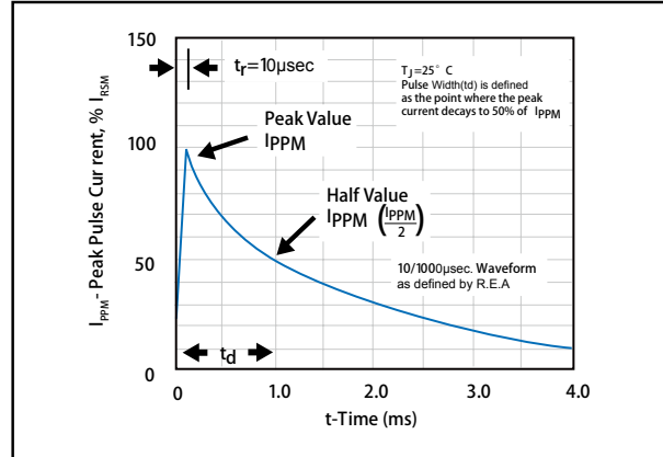
Figure 4 - Pulse Waveform
