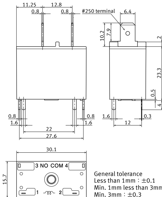
External dimensions
