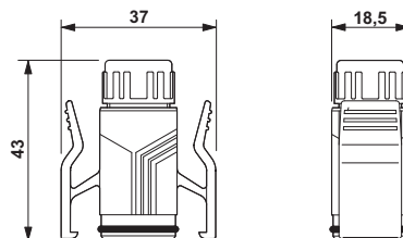
Dimensioned drawing
