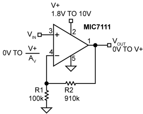
Figure 3. Noninverting Amplifier
