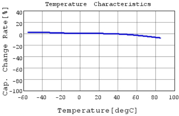
GRM155R61E102KA01 C-Temp. capchange, DC0.0V,
