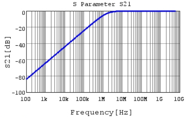
GRM155R61E102KA01 S21 DC0V, 25degC
