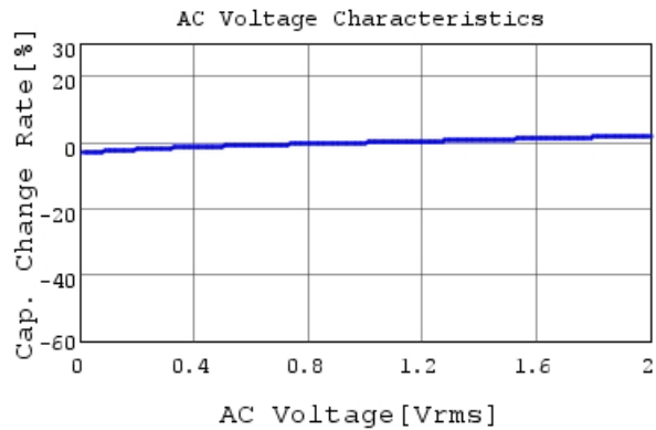
GRM155R61E102KA01 C-AC Voltage capchange, Dc
