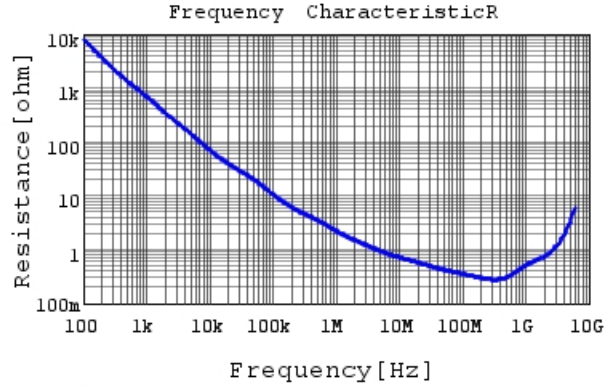
GRM155R61E102KA01 R DCOV, 25degC
