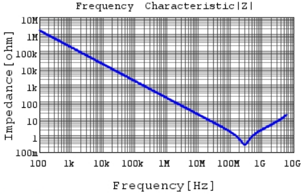
GRM155R61E102KA01 |Z| DCOV, 25degC
