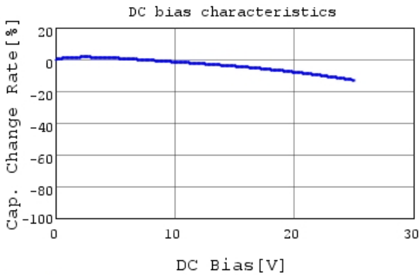
GRM155R61E102KA01 C-DC bias capchange, 25.0c
