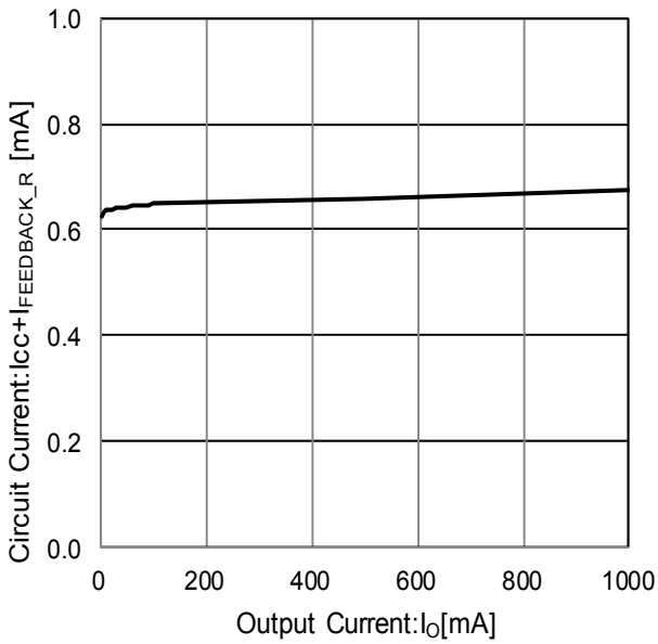
Figure 20. Circuit Current vs Output Current ( I_o = 0\text{mA} \rightarrow 1000\text{ mA} ) ( I_{FEEDBACK\_R} \cong 75\mu\text{A} )
