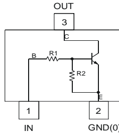
Device Schematic
