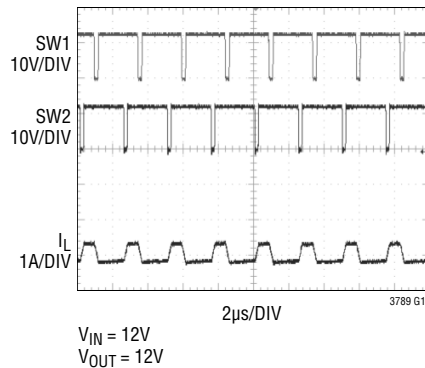
Pulse-Skipping Mode
