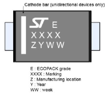
Figure 19. Marking layout
