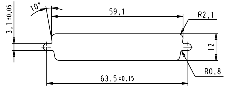
Panel cut out 1:1
