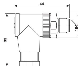
Dimensioned drawing
