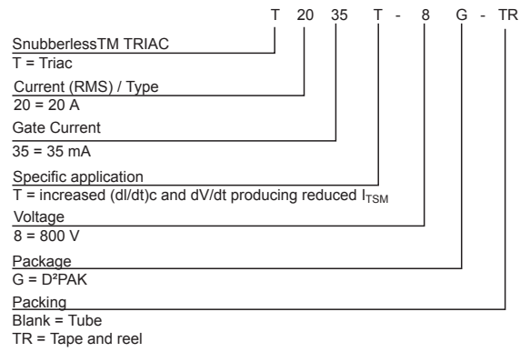
Figure 16. Ordering information scheme
