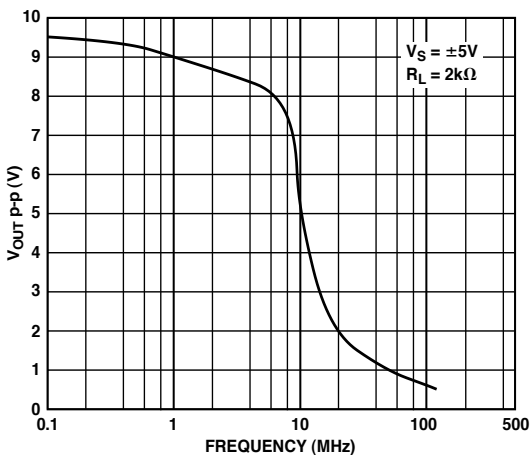
Figure 24. Output Voltage Swing vs. Frequency
