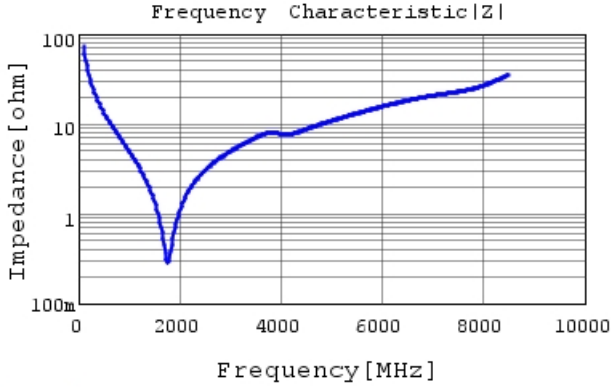
GCM1555C1H220JA16 |Z| DC0V, 25degC
