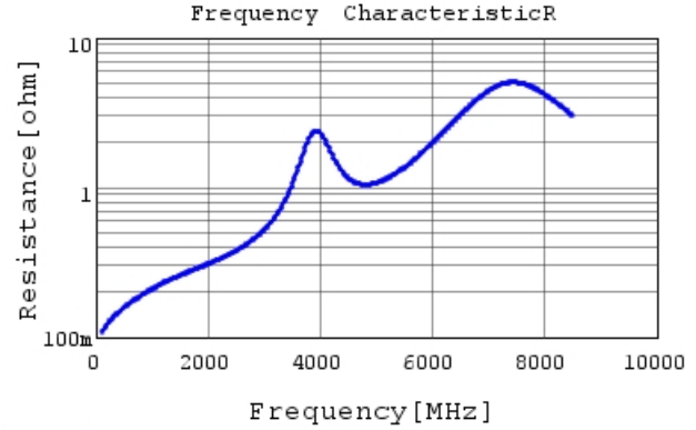
GCM1555C1H220JA16 R DC0V, 25degC
