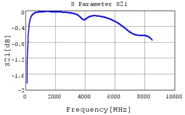
GCM1555C1H220JA16 S21 DCOV, 25degC
