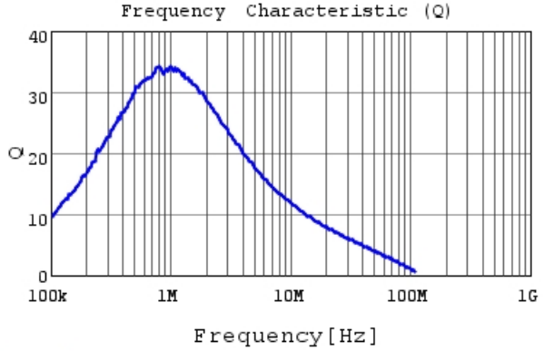
1286AS-H-R47M Q
