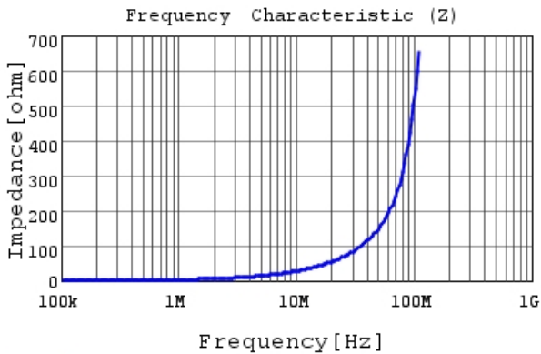
1286AS-H-R47M |Z|
