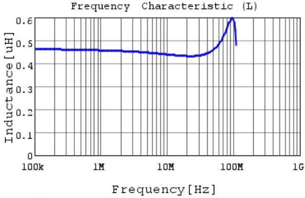
1286AS-H-R47M L
