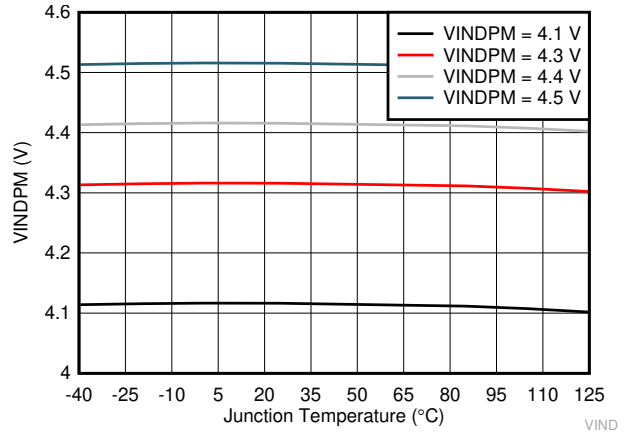
Figure 7-8. VINDPM vs Junction Temperature
