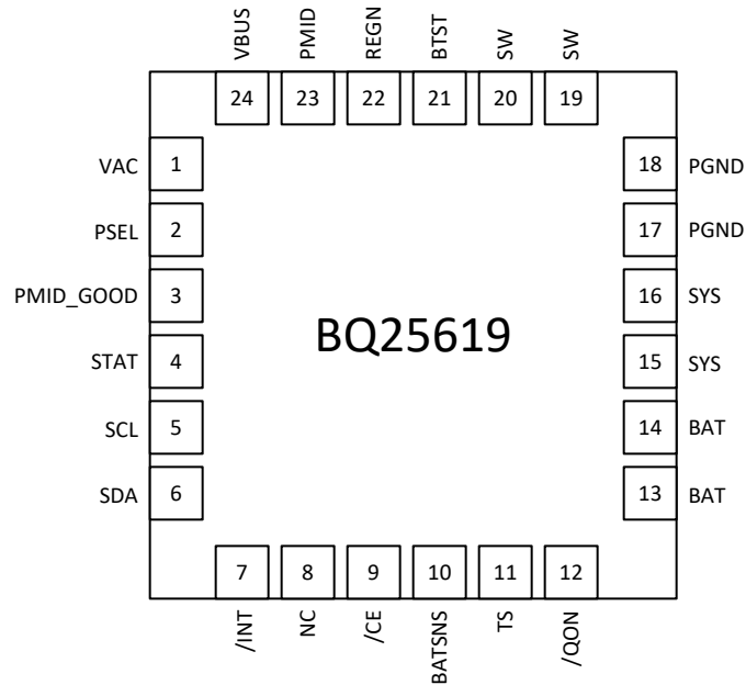
Figure 6-2. BQ25619 RTW Package 24-Pin WQFN Top View
