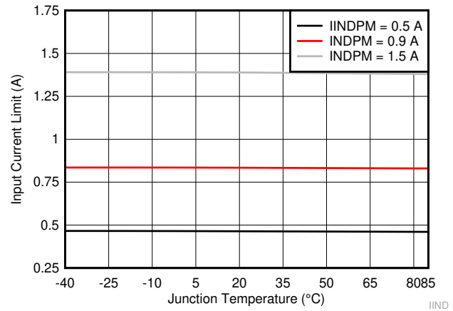
Figure 7-10. Input Current Limit vs Junction Temperature
