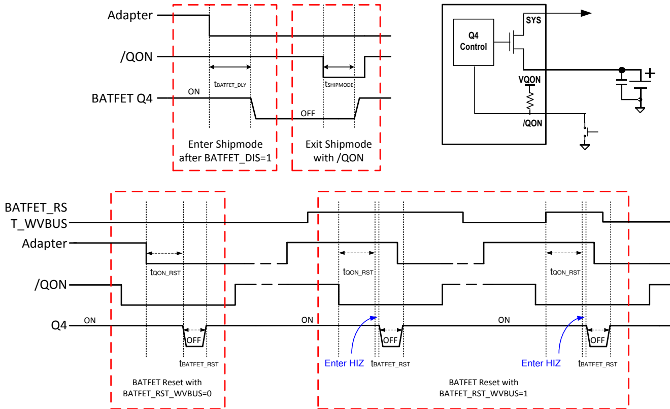
Figure 8-6. QON Timing
