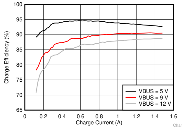
Figure 7-2. Charge Efficiency
