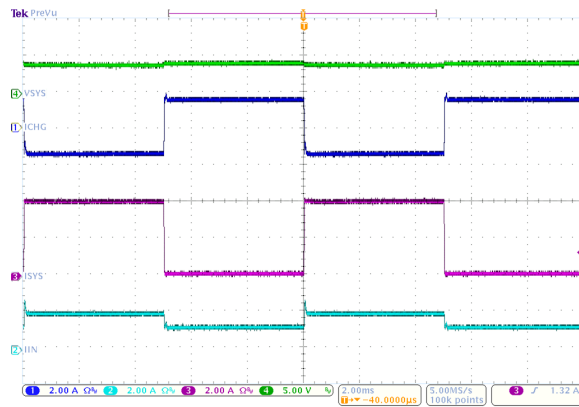
Figure 9-8. System Load Transient Response
