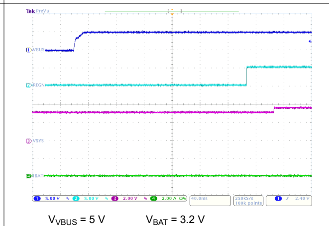
Figure 9-5. Power Up with Charge Disabled
