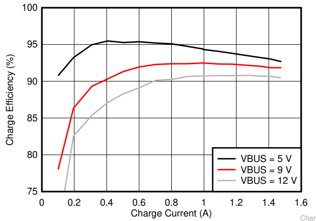
Figure 7-1. Charge Efficiency
