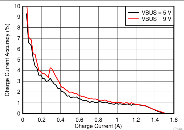
Figure 7-5. Charge Current Accuracy
