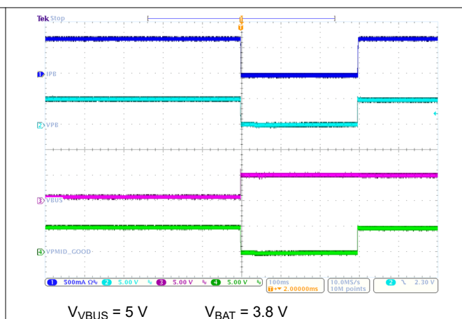
Figure 9-3. VBUS Plugged In with Boost Mode Enabled
