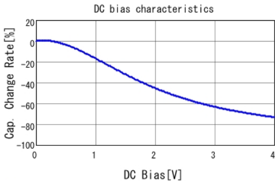
■ GRM155R60G475ME47 C-DC bias capchange, 25.0degC, ACO.
