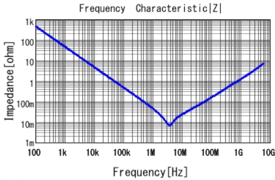
■ GRM155R60G475ME47 |Z| DCOV, 25degC
