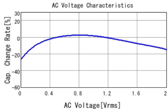
■ GRM155R60G475ME47 C-AC Voltage capchange, DCOV, 25.0d
