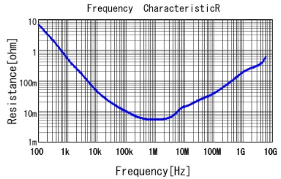
■ GRM155R60G475ME47 R DCOV, 25degC
