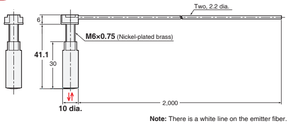
23-H E32-C91N 2M (Free Cutting) + E39-F18
