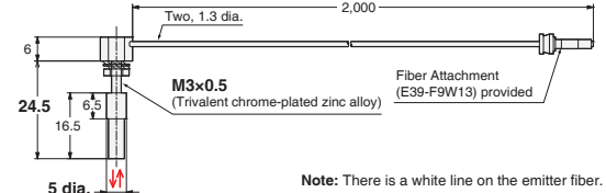
23-C E32-C21N 2M (Free Cutting) + E39-F3A-5
