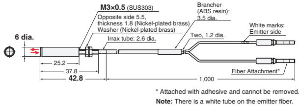
23-E E32-C31 2M (Free Cutting) + E39-F3B
