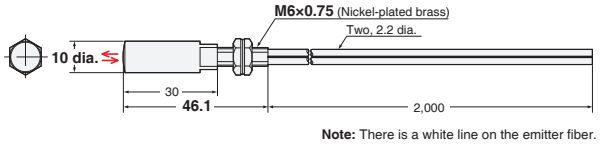
23-H E32-C91N 2M (Free Cutting) + E39-F18
