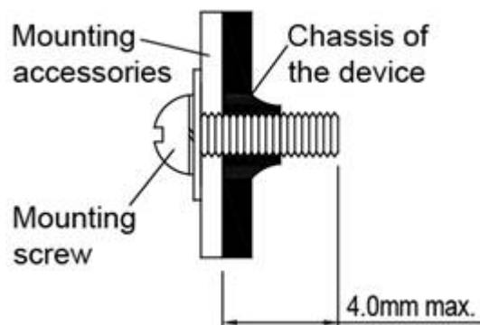
Fig. 4 Mounting Screw
