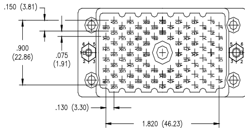
90 PIN PLUG
