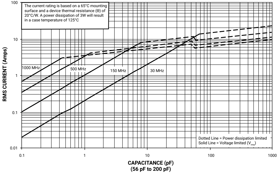
CURRENT RATING VS. CAPACITANCE SERIES 100, CASE B
