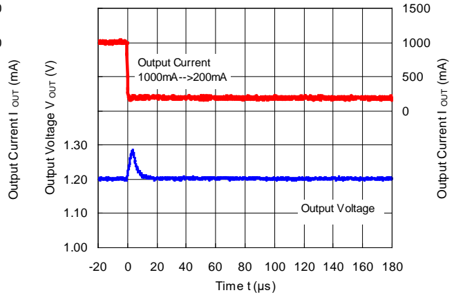
RP506Kxx1A/B/C ( V_{IN} = 3.6\text{ V} , V_{OUT} = 1.2\text{ V} )
