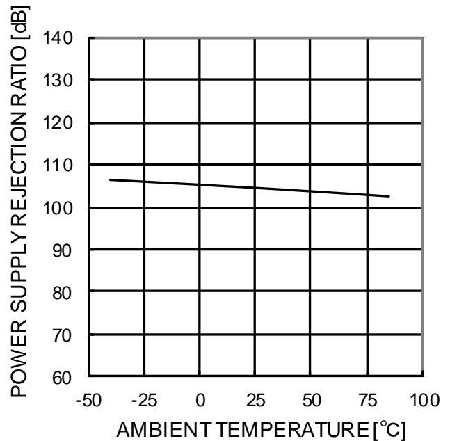
Figure 25. Power Supply Rejection Ratio - Ambient Temperature
