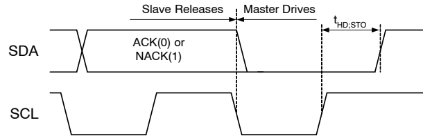
Figure 16. STOP Bit
