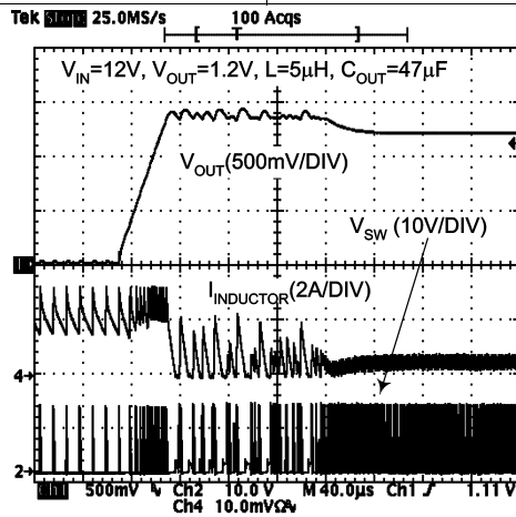
Figure 23. Short-Circuit Release
