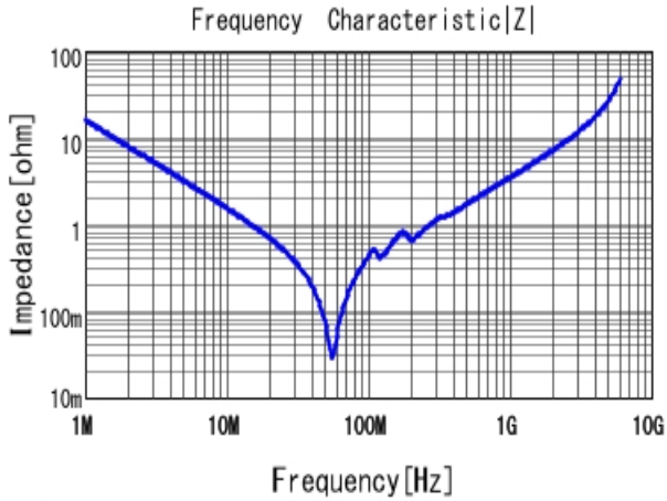
■ GRM3195C2A103JA01 |Z| DCOV, 25degC
