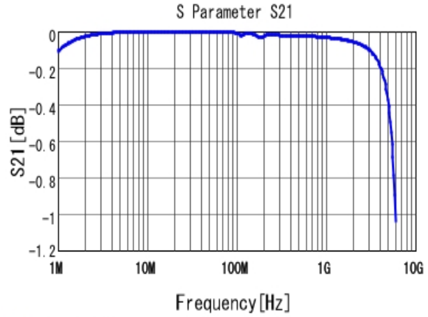
■ GRM3195C2A103JA01 S21 DCOV, 25degC
