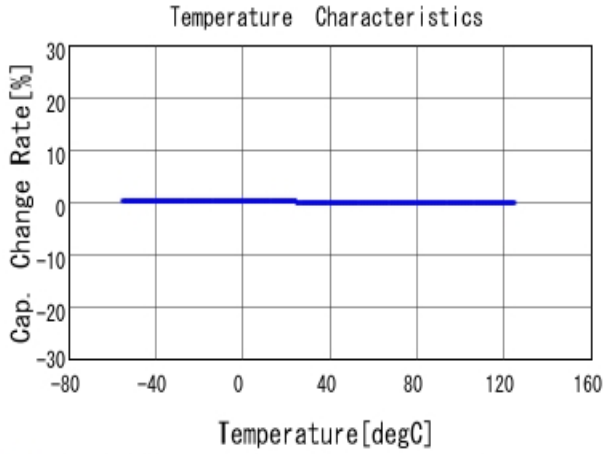
■ GRM3195C2A103JA01 C-Temp. capchange, DCOV, AC1Vrms
