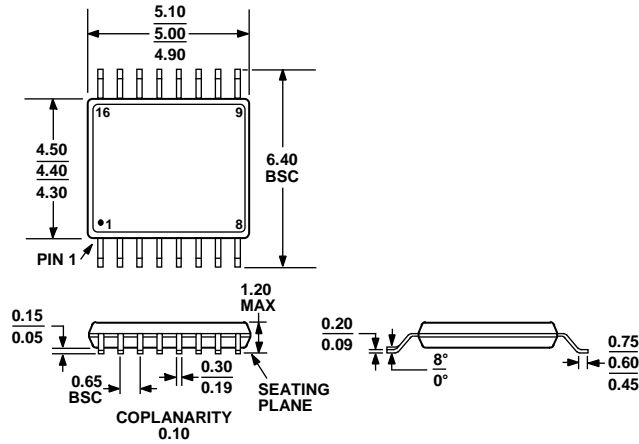
COMPLIANT TO JEDEC STANDARDS MO-153-AB Figure 2. 16-Lead Thin Shrink Small Outline Package [TSSOP] (RU-16) Dimensions shown in millimeters
