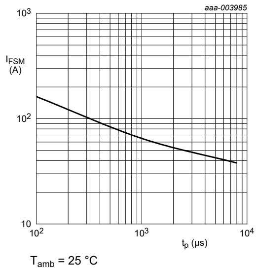
Fig. 7. Non-repetitive peak forward current as a function of pulse duration; typical values
