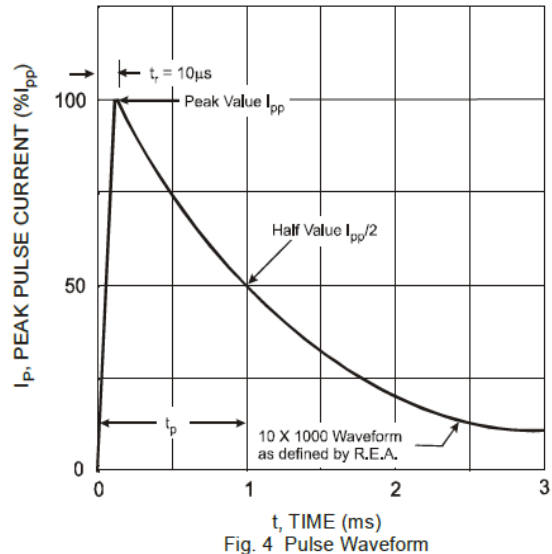
Fig. 4 Pulse Waveform
