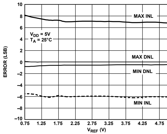
Figure 25. INL and DNL Error vs. V_{REF}
