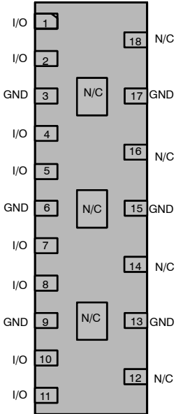
Figure 2. Pin Configuration
