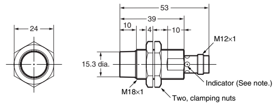
E2A-M18KN16-M1-□□/E2A-S18KN16-M1-□
