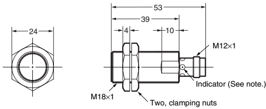
E2A-M18KS08-M1-□□/E2A-S18KS08-M1-□
