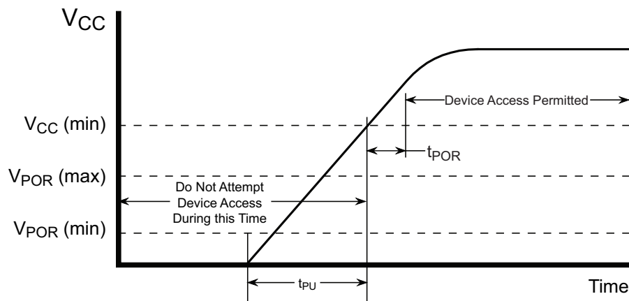
Figure 11-2. Power-Up Timing
